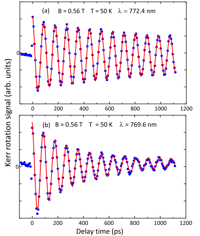
FIG. 2. Photoinduced Kerr rotation signals for sample B, in a magnetic field B = 0.56 T, at 50 K. Pump and probe energies are tuned to the wavelength (a) \lambda = 772.4 nm, D^0X transition; (b) \lambda = 769.6 nm, X transition. Blue full disks: experimental data; red continuous lines: fits with Eq. (2).
