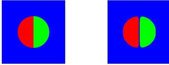
FIGURE 7. Illustration of the lack of lower semicontinuity when the triangle inequality does not hold. Initialisation (left) and obtained result (right).
