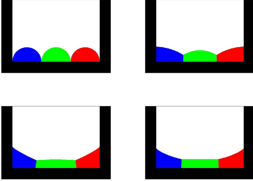
FIGURE 6. Partition with 5 phases and volume constraint: initialization (top left), obtained result in case (a) (top right), obtained result in case (b) (bottom left), obtained result in case (c) (bottom right).
