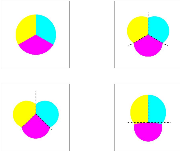
FIGURE 5. Illustration of Herring's law. Initialisation (top left), obtained result in case (a) (top right), obtained result in case (b) (bottom left), obtained result in case (c) (bottom right). The theoretical angles at the junction point are displayed in dashed line.
