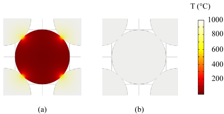
Fig. 11 FEM temperature maps in metallic powder particles 100 \mu\text{m} in diameter heated by hot spots ( T \approx 1000^\circ\text{C} ) at their periphery, showing temperature homogenization in the particles within milliseconds. (a) Temperature map at t = 0 . (b) Temperature map at t = 4 \times 10^{-3} s (Collard et al. 2017).
