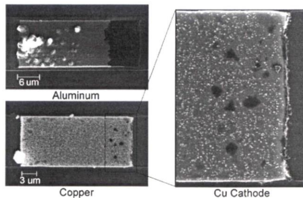
Fig. 2 Al and Cu conductor segments submitted to a current density of 6 \times 10^5 A/cm 2 in the following conditions: 250^\circ\text{C} – 336 h for Cu, 200^\circ\text{C} – 500 h for Al (electron sense: from right to left). Note the depletion of matter at the cathode and its accumulation at the anode (Frankovic 1996).
