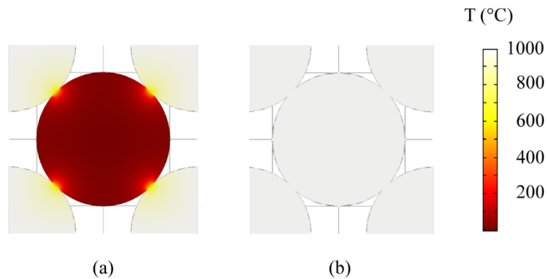
Fig. 11 FEM temperature maps in metallic powder particles 100 µm in diameter heated by hot spots ( T \approx 1000\text{C}^\circ ) at their periphery, showing temperature homogenization in the particles within milliseconds. (a) Temperature map at t = 0 . (b) Temperature map at t = 4 \times 10^{-3} s (Collard et al. 2017).
