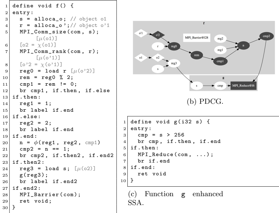
Fig. 3: Enhanced SSA form of the MPI code Figure 1a and its corresponding PDCG.
