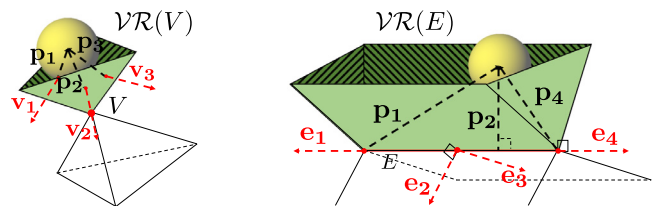
Fig. 15. On the left, \mathcal{VR}(V) normals \mathbf{v}_1 , \mathbf{v}_2 and \mathbf{v}_3 are elucidated along with the approaching particle's corresponding vectors \mathbf{p}_1 , \mathbf{p}_2 and \mathbf{p}_3 for dot products calculations. On the right, \mathcal{VR}(E) normals \mathbf{e}_1 , \mathbf{e}_2 , \mathbf{e}_3 and \mathbf{e}_4 are elucidated along with the approaching particle's corresponding vectors \mathbf{p}_1 , \mathbf{p}_2 and \mathbf{p}_4 for dot product calculations. \mathbf{p}_3 is equal to \mathbf{p}_2 .
