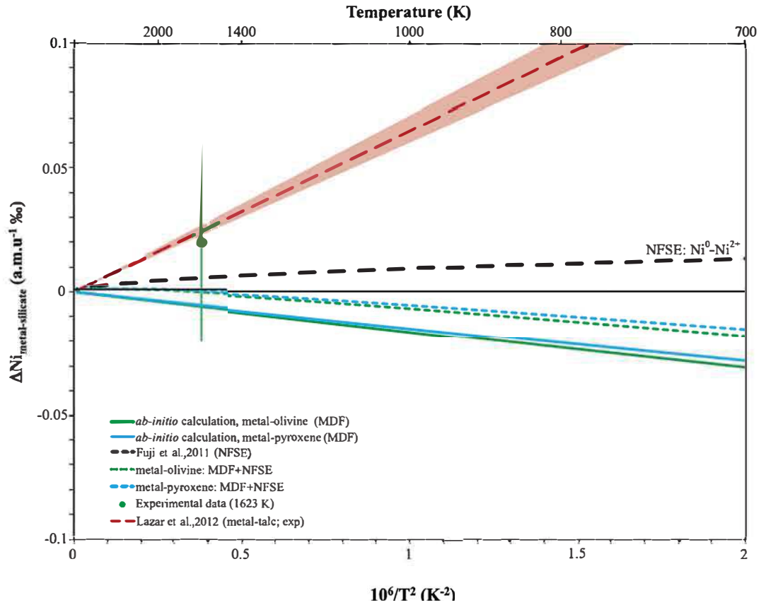
Fig. 5. Evolution of the metal silicate isotope fractionation factor at equilibrium ( \Delta\text{Ni} in \text{a.m.u.}^{-1} ) as a function of temperature. The metal olivine/pyroxene fractionation (Mass dependent fractionation, MDF) are found to be negative and extrapolation with temperature show a weak dependency. Experimental data on metal talc (Lazar et al., 2012) do not match our theoretical calculations. Conversely, our experimental data points on metal silicate melt at high temperature agrees with the calculations within error bars. Contribution of nuclear field shift effects (NFSE) has been calculated (Fuji et al., 2011) and is not significant relative to the total fractionation. Width of this curve shows the variability of this process for the different isotopes ratios.
