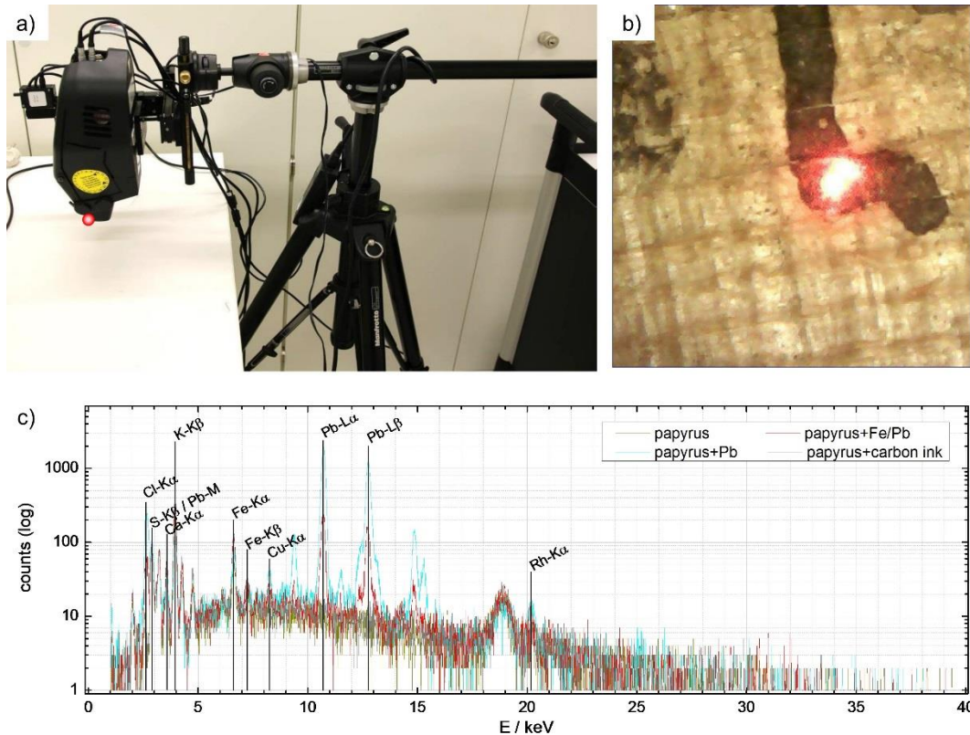
Figure 2: a) Mobile XRF spectrometer ELIO, b) laser spot on fragment and c) measured spectra. For element-sensitive mapping, a proper energy bandwidth around one peak is selected
