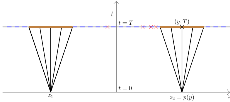
Figure 5: Illustration of (t, x) \rightarrow S_t^+S_T^-(u^T)(x) , p^{-1}(X(S_T^-(u^T))) \subset X(S_T^+S_T^-(u^T)) (—), X(S_T^+S_T^-(u^T)) \setminus p^{-1}(X(S_T^-(u^T))) (-) and discontinuous points of S_T^+S_T^-(u^T) ( \times ). Here, y \in X(S_T^+S_T^-(u^T)) \setminus p^{-1}(X(S_T^-(u^T))) , p(y) is defined in (29) and at any discontinuous points (z_k)_{k \in \mathbb{N}} of S_T^-(u^T) verifying S_T^-(u^T)(z_k^-) < S_T^-(u^T)(z_k^+) , a rarefaction wave is created at time t = 0 .
