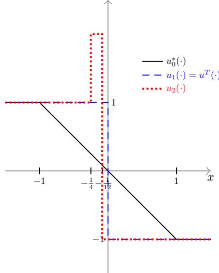
Figure 1: Three initial data u_0^*(-) , u_1(- -) and u_2(\cdot \cdot \cdot) leading to a attainable target u^T(\cdot) := \mathbb{1}_{(-\infty, 0)}(\cdot) - \mathbb{1}_{(0, +\infty)}(\cdot) at time T = 1 along forward entropic evolution.
