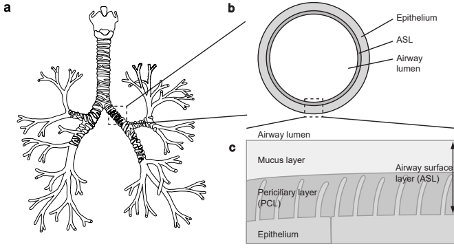
Figure 1: a) Picture of a lung cast: bronchial region. b) Schematic transverse view of an airway, with the different layers surrounding the lumen of the airway. c) The cilia penetrate in the ASL and generate the displacement of the mucus.
