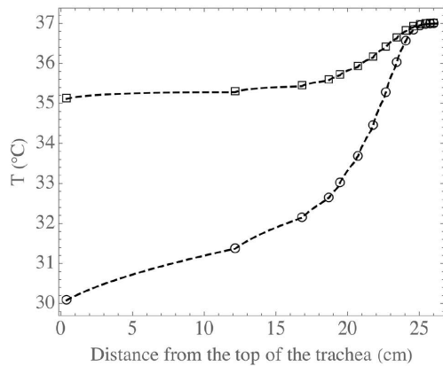
Fig 2a Average temperature of the air at the end of inspiration (○) and expiration (□) on a flow cross-section as a function of the distance from the top of the trachea, at rest, with T^{\text{in}} = 30^\circ\text{C} and \text{RH}^{\text{in}} = 0.8 .
