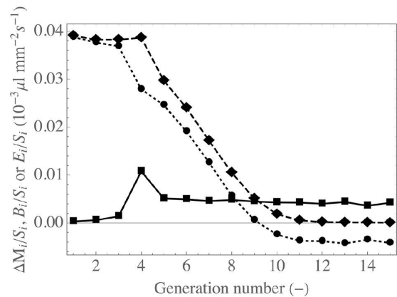
Fig 2b Magnitude of the mechanisms controlling the bronchial mucus balance, by unit surface S_i , with T^{\text{in}} = 34^\circ\text{C} and \text{RH}^{\text{in}} = 0.95 . (■): mucus displacement contribution; (◆): evaporation contribution; (●): other control mechanisms contribution.
