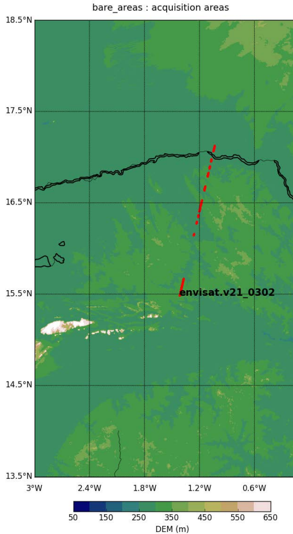
Fig. 1. Locations of the selected altimetry data along ERS-2/ENVISAT/SARAL ground-track 0302 in the Gourma region of Mali.
