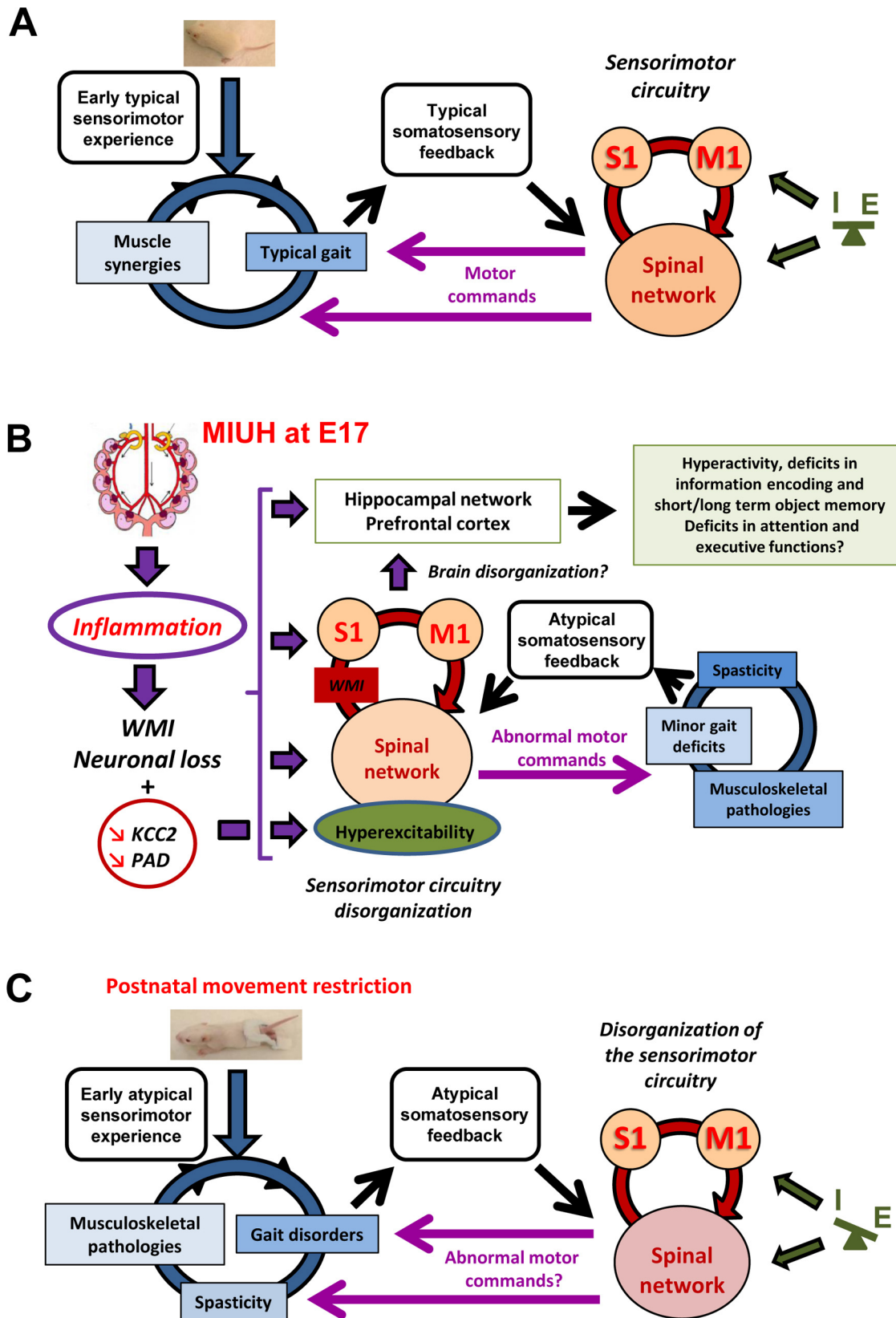
Fig. 2. Illustration of the putative interactions and processes underlying the emergence of movement disorders and brain plasticity. A. Schematic representation of the putative interactions between the different variables assessed (locomotion, musculoskeletal tissues, Hoffman-reflex, somatosensory and motor representations of the hind limb and excitation-inhibition neurotransmission in the sensorimotor cortex) that may occur during typical sensorimotor development in control rats. Daily activities provide early typical sensorimotor experience that allows muscle synergies and typical gait to interplay harmoniously. Normal movements during typical gait produce typical sensorimotor feedback to the immature brain, contributing to the development and refinement of connections, maps and functions (e.g., normal motor command to muscles that in turn contribute to muscle synergies and typical movements in a virtuous self-perpetuating cycle). Excitation-inhibition balance also participates in the refinement of neural maps and connections. S1: primary somatosensory cortex; M1: motor cortex. B. Schematic illustration of the detrimental impact of mild intrauterine hypoperfusion (MIUH) on neuromuscular interplay and brain disorganization. MIUH induces early inflammation and likely enhances immunoreactions that lead to diffuse WMI (loss of
