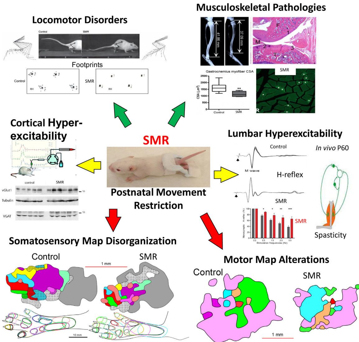
Fig. 3. Schematic summary of the variety of symptoms reproduced in our rat model of developmental coordination disorder based on early movement restriction. Such a hind-limb immobilization from birth to 1 month provides atypical sensorimotor experience during development. See text in “Animal model of developmental coordination disorder” for details. SMR: sensorimotor restriction.
