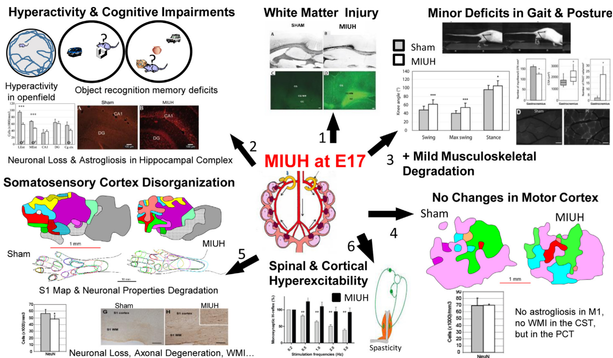
Fig. 1. Schematic summary of the diversity of symptoms that successfully reproduces our rat model of encephalopathy of prematurity, based on mild intrauterine hypoperfusion (MIUH) at embryonic day 17 (E17). See “Animal model of cerebral palsy” for details. WMI: white matter injury; S1: primary somatosensory cortex; CST: corticospinal tractus; PCT: pontocerebellar tractus.
