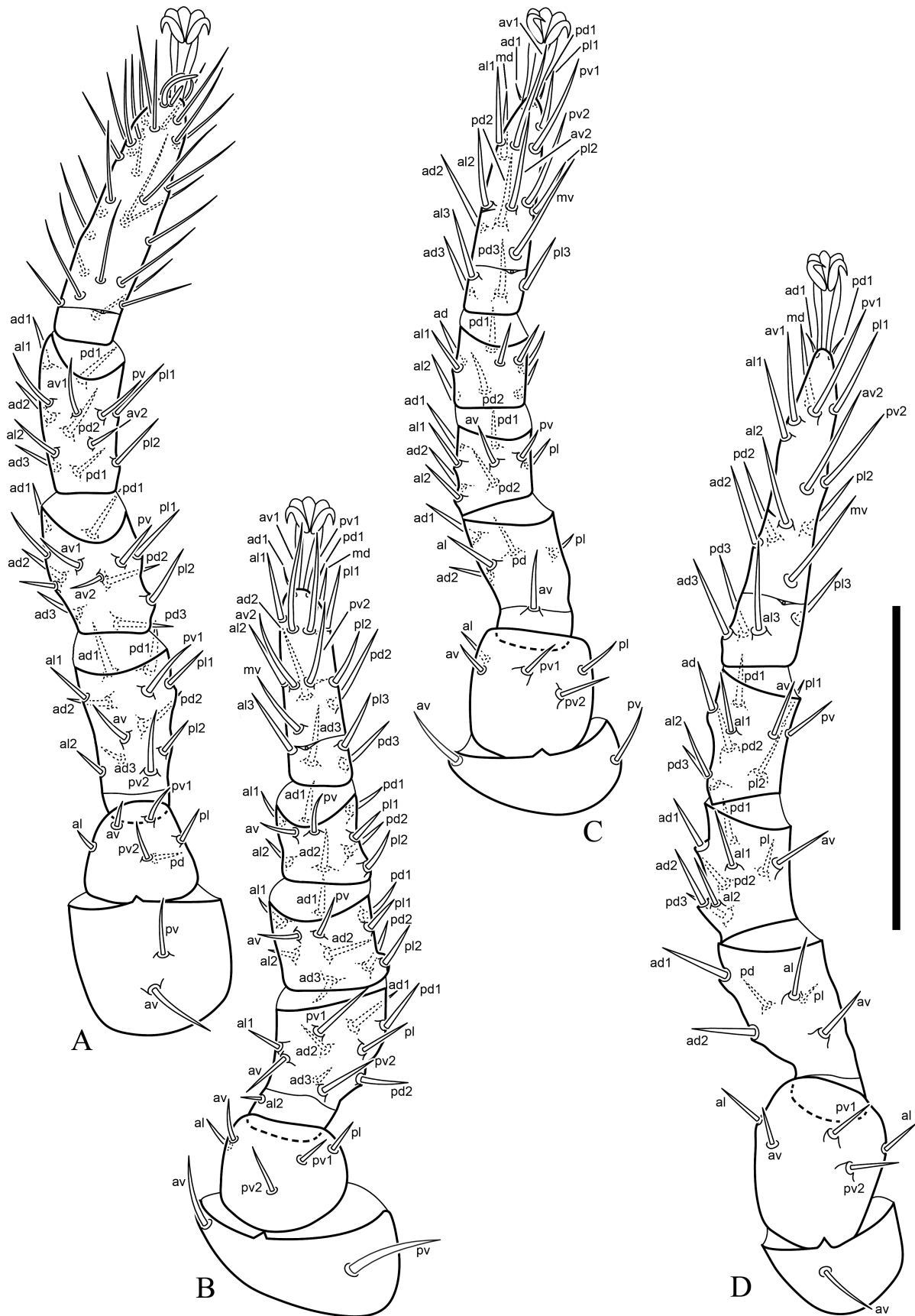
Figure 4 Proctolaelaps sibiriensis (Davydova, 1988), female: A – leg I, ventral view; B – leg II, ventral view; C – leg III, ventral view; D – leg IV, ventral view. Scale bar: 100 μm.
