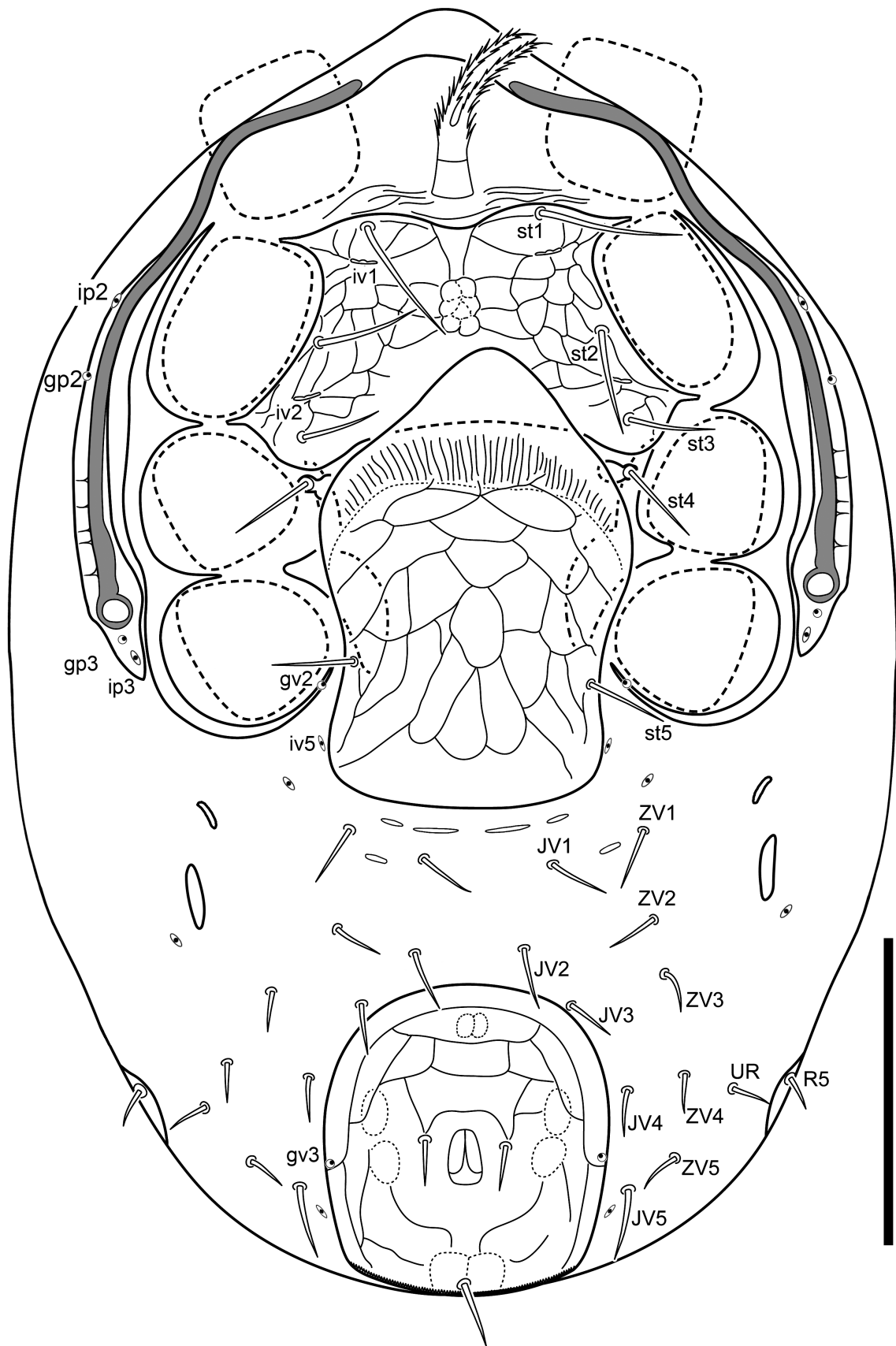
Figure 2 Proctolaelaps sibiriensis (Davydova, 1988), female: idiosoma, ventral view. Scale bar: 100 µm.
