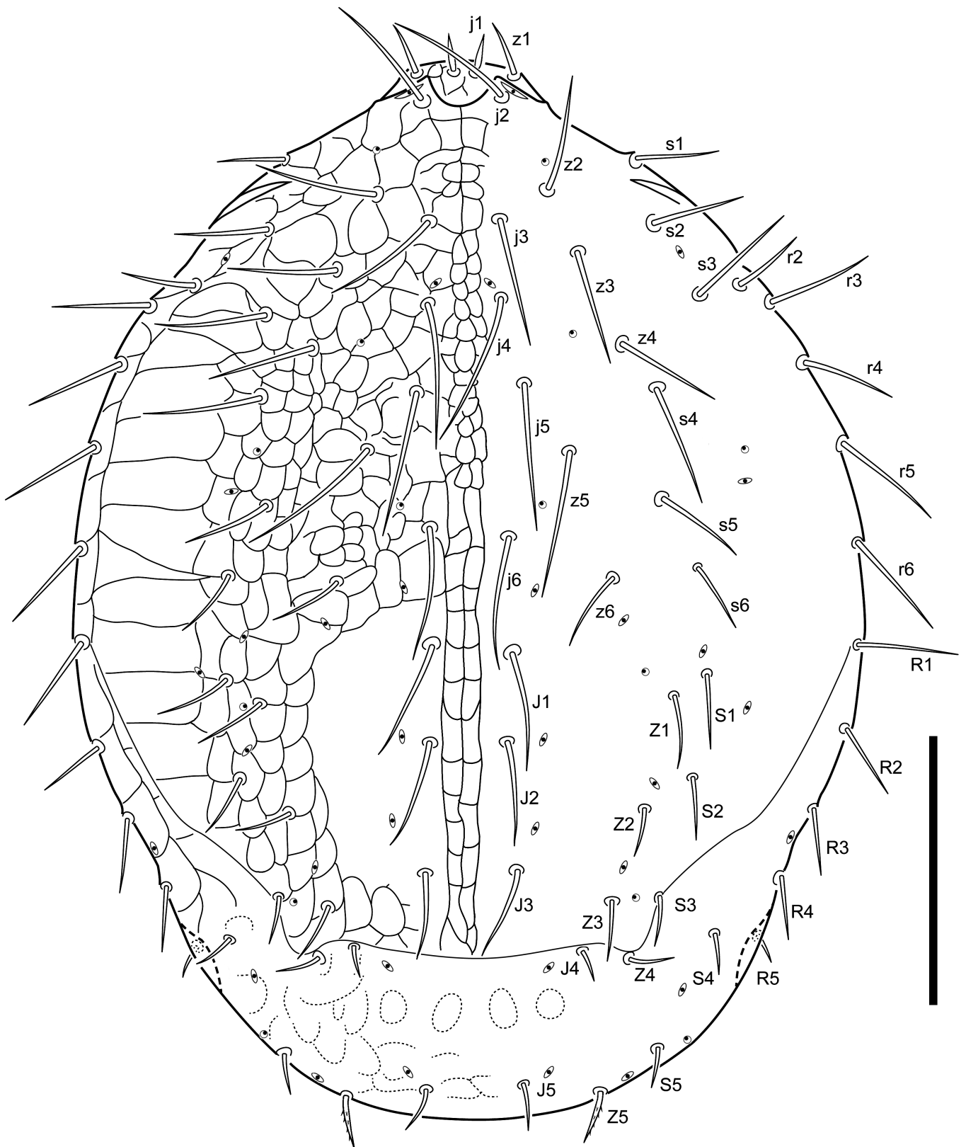
Figure 1 Proctolaelaps sibiriensis (Davydova, 1988), female: idiosoma, dorsal view. Scale bar: 100 \mu m.
