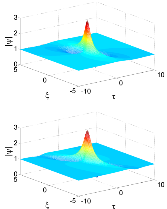
FIG. 2. (Color online) Typical rogue soliton states. Top, focusing regime \sigma = 1 , \kappa = 0.5 and a = 1 , \omega = 0 . Bottom, defocusing regime \sigma = -1 , \kappa = 0.5 and a = 1 , \omega = 4 .
