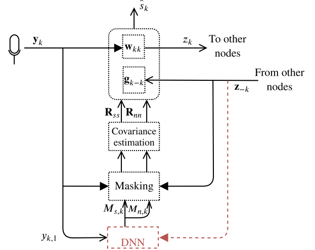
Fig. 2. Expansion of the iterated step in Figure 1. Red arrows are the modifications brought to DANSE. Plain arrows represent vectors, simple ones represent scalars.
