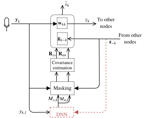
Fig. 2. Expansion of the iterated step in Figure 1. Red arrows are the modifications brought to DANSE. Plain arrows represent vectors, simple ones represent scalars.
