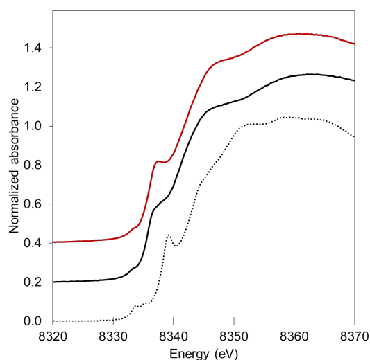
Figure 6. XANES spectra of \text{NiL}^{3\text{S}}(\text{OH}_2) (black line, offset of 0.2), \text{NiL}^{3\text{S}}(\text{OH}) (red line, offset of 0.4) and \text{Ni}(\text{N}_2\text{S}_2) (dashed line, offset of 0.0)
