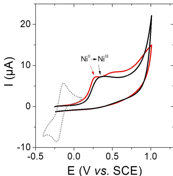
Figure 8. Cyclic voltammograms at 100 mV/s of NiL 3S (OH 2 ) (black) and NiL 3S (OH) (red) at 570 µM in HEPES buffer (20 mM, pH 7.4 and 9.5 respectively, [NaCl] = 100 mM), (dotted gray) CV at 100 mV/s of the Ru III (NH 3 ) 6 Cl 3 probe
