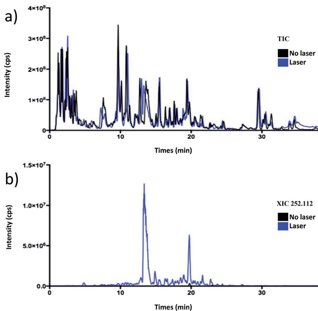
Figure 3: a) Total ion chromatogram of the AIF-MS/MS of a digest of 3 proteins during 50 min with a gradient of acetonitrile 20–45 % and (b) extracted chromatogram of the reporter ion m/z 252, with (blue) or without (black) laser. Reproduced with permission from Ref 31
