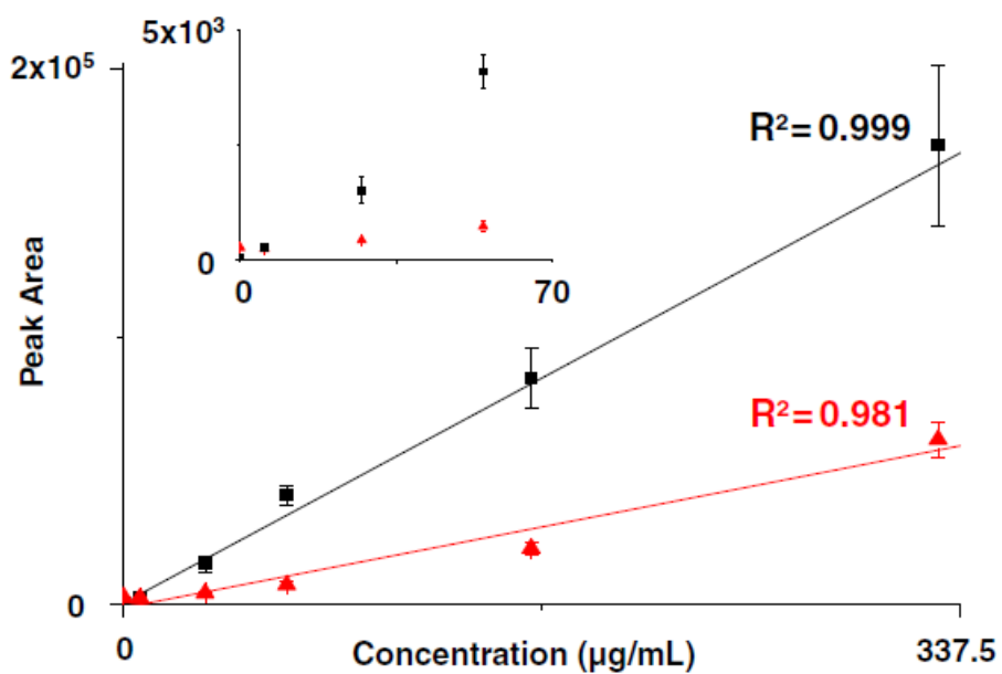
Figure 5: Calibration curves for the most intense specific transition for chromophore-derivatized proteotypic C4b binding protein alpha chain peptide monitored by use of photo-SRM (squares) and SRM (triangles). Inset shows low concentration data (0, 6.75, 33.75, and 67.5 \mu\text{g mL}^{-1} ). Reproduced with permission from Springer Nature Ref 34 Copyright 2013 American Chemical Society
