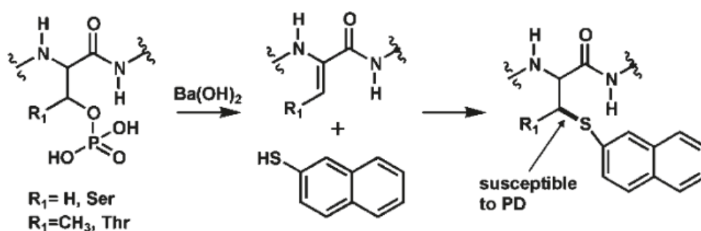
Scheme 5. Dephosphorylation and derivatization by Naphthalenethiol. Reproduced with permission from Ref 43 Copyright 2011 American Chemical Society
