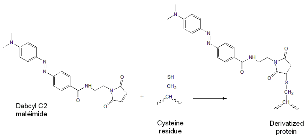
Scheme 2. Reaction of cysteine with Dabcyl C2 maleimide.
