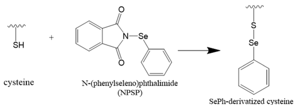
Scheme 3. Reaction of Free Thiols with N-(Phenylseleno)phthalimide. Reproduced with permission from Ref 36 Copyright 2016 American Chemical Society
