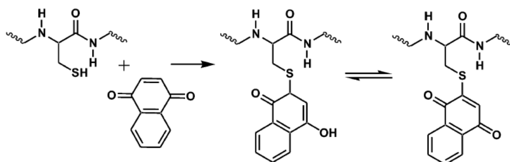
Scheme 4. Modification of cysteine by quinone. Reproduced with permission from Ref 37 Copyright 2010 American Chemical Society
