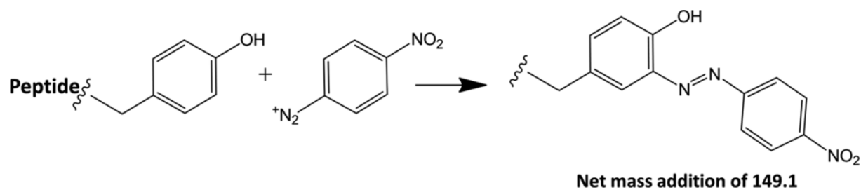
Scheme 1. Reaction Schematic of Diazonium Coupling with Tyrosine. Reproduced with permission from Ref 27 Copyright 2014 American Chemical Society
