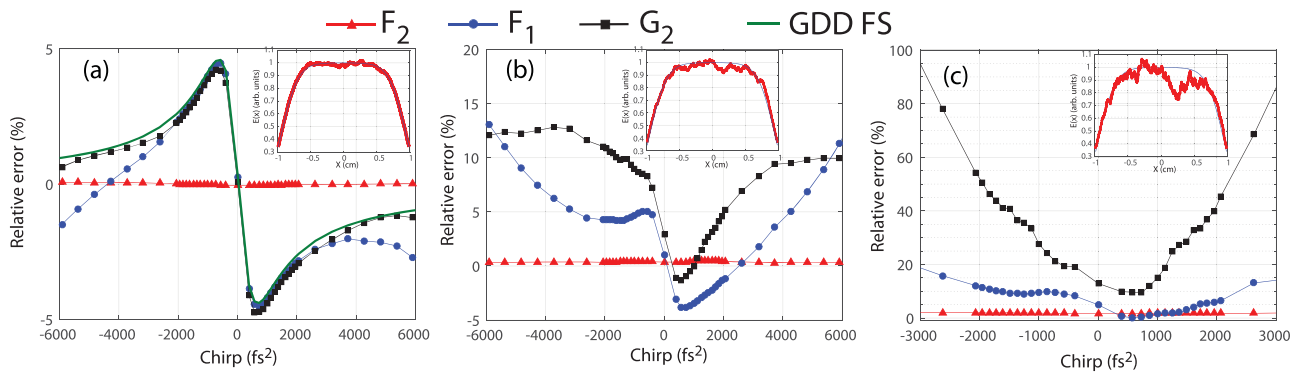
FIG. 11. Relative error made by the fit as a function of the initial chirp in the presence of a low (a), intermediate (b), and strong (c) noise in the spatial profile for a fused silica 160° biprism. The central wavelength of the pulse is 2 μm, and the FTL pulse duration is 60 fs. The associated spatial electric field profile is shown in the subpanels.
