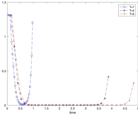
Figure 5: Error between dynamical optimal triple and static one (Relaxation case)
