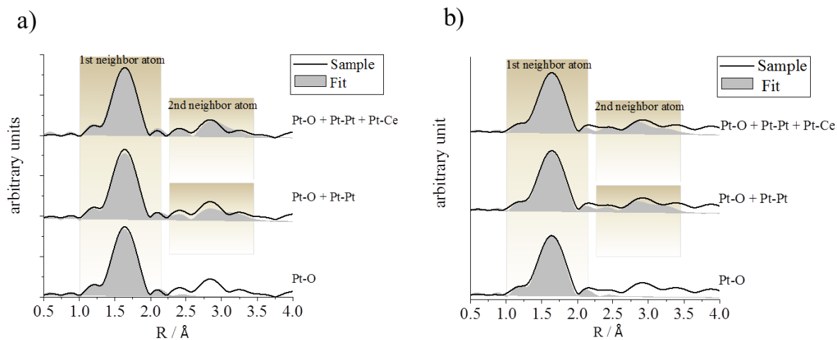
Fig. SI5 Evolution of the EXAFS fit (filled area) and FTs (solid line). a) 1% Pt/CeO 2 as-synthesized, b) 1% Pt/CeO 2 300 H 2 . Contributions of Pt-O, Pt-Pt and Pt-Ce bonds are specified in the corresponding fits.
