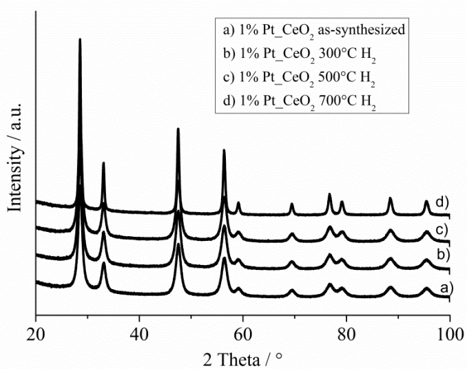
Fig. 1. XRD pattern of the one-step synthesized samples treated under hydrogen at different temperatures.
