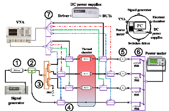
Fig. 11. Schematic of RF/thermal stress test setup: ① power amplifier, ② coupler, ③ four-way power divider, ④ SPDT, ⑤ attenuators, ⑥ SP4T 50Ω RF load terminations ⑦ SP4T.
