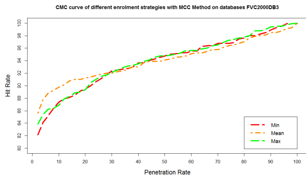
Figure 6. CMC identification performance on database FVC2000DB3 using MCC method
