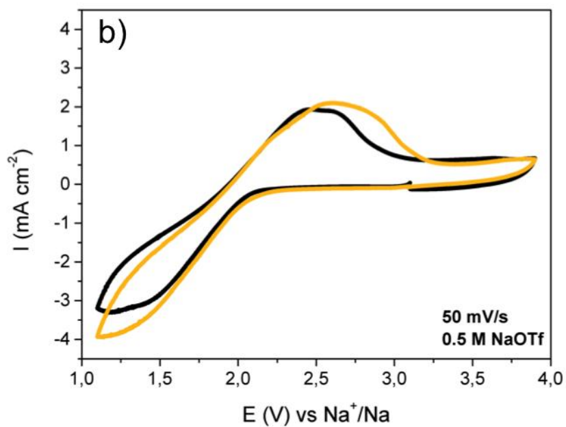
Figure S4: SEM image of Au-coated GDL fibers (20-30 nm) (a). Cyclic voltammograms of oxygen reduction on GDL (black) and Au-coated GDL (yellow) surfaces at 50 mV/s in DGME using 0.5M NaOTf as conductive salt (b).
