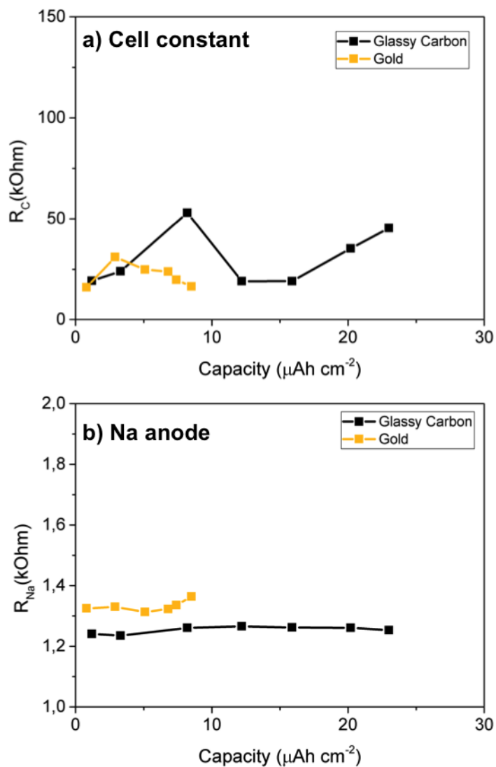
Figure S2: Fitted resistance evolution based on of the cell constant (a) and the Na anode (b) when using an Au (yellow line) and GC (black line) working electrode during discharge at 100 \mu\text{A/cm}^2 in DGME (0.5 M NaOTf).
