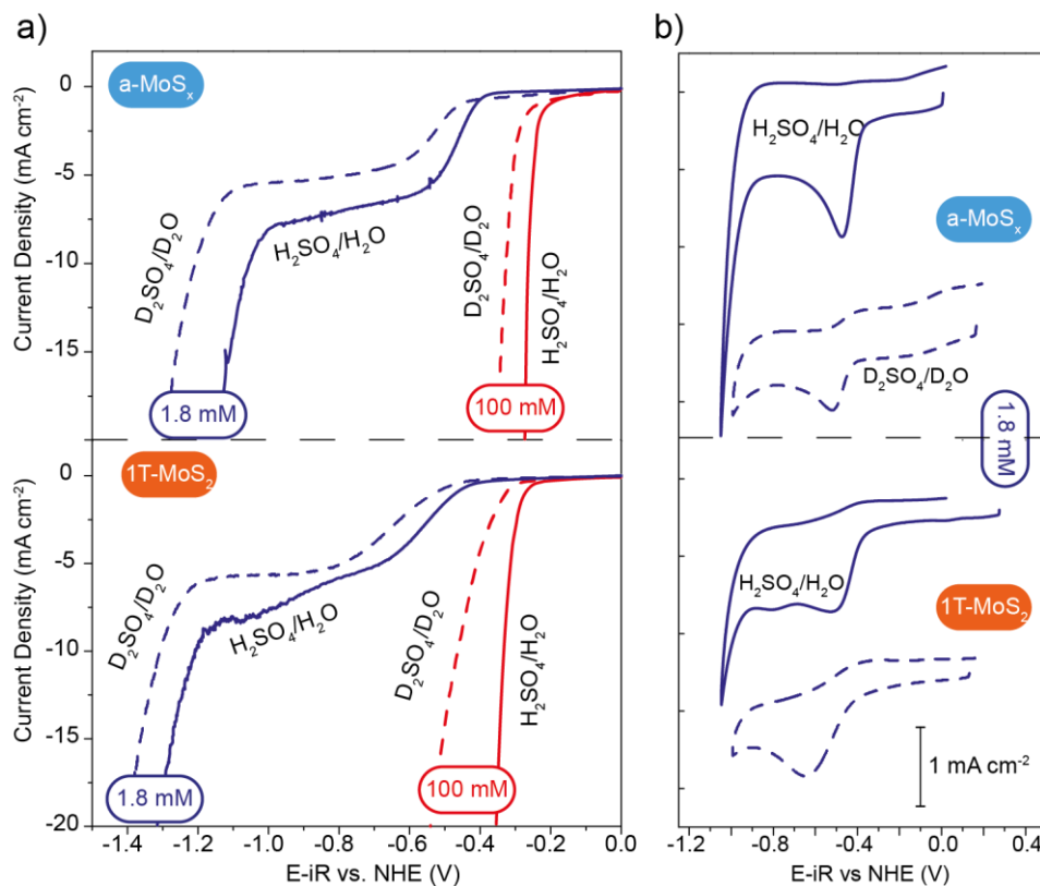
Figure 6. a) Polarization curves recorded in normal (solid lines) or deuterated electrolytes (dashed lines) 100 mM acid (red) and 1.8 mM (blue) at 20 mV s -1 using a RDE at 1,600 rpm and b) corresponding static CVs recorded in the 1.8 mM acid electrolytes at 100 mV s -1 over amorphous MoS 2 (top) and exfoliated 1T-MoS 2 (bottom) electrodes. In b), each tick on the left axis corresponds to 1 mA cm -2 .
