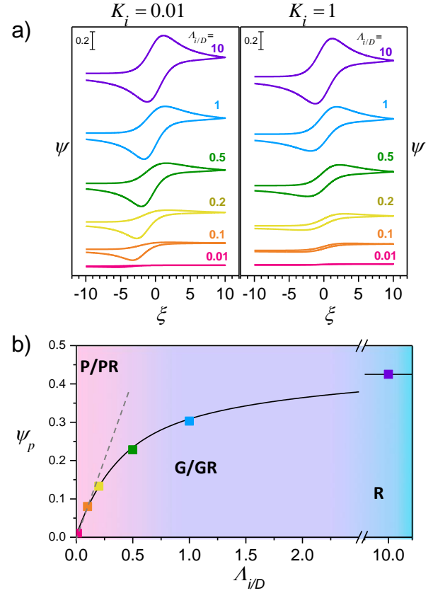
Figure 10. (a) Simulated CVs as function of \Lambda for K = 0.01 (left) and K = 1 (right). \Lambda = 0.01 (red), 0.1 (orange), 0.2 (yellow), 0.5 (green), 1 (blue), 10 (purple). (b) Simulated dimensionless plateau or peak current as function of \Lambda for K = 1 .
