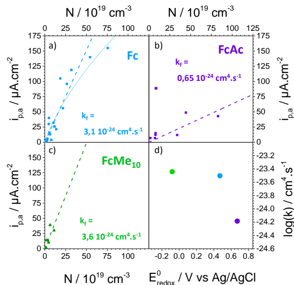
Figure 7. Variation of the anodic plateau current of Fc (a), FcAc (b) and FcMe10 (c) with the doping density of the WO_3 electrodes. (d) Correlation between the apparent rate constant and the standard potential of the redox probes.
