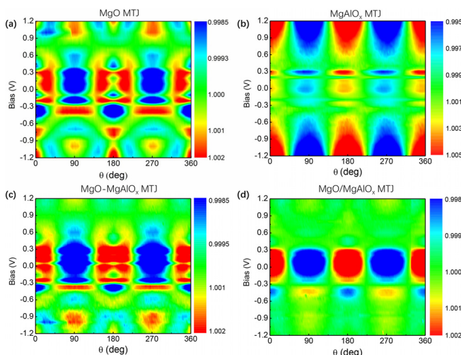
FIG. 3. Normalized dV/dI as a function of bias voltage and angle \theta for MgO (a), \text{MgAlO}_x (b), MgO-MgAlO x (c), and MgO/MgAlO x (d) MTJs, respectively. The magnitude of dV/dI is shown by the color.
