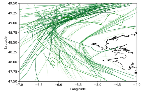
Fig. 9. AIS tracks that cannot be mapped to maritime routes, hence cannot be monitored by DBSCAN-based methods. In the test set that comprises only cargo and tanker vessels (from March 21 to March 31, 2017), such tracks account for 13% of all AIS tracks.
