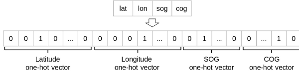
Fig. 1. “Four-hot” vector.
