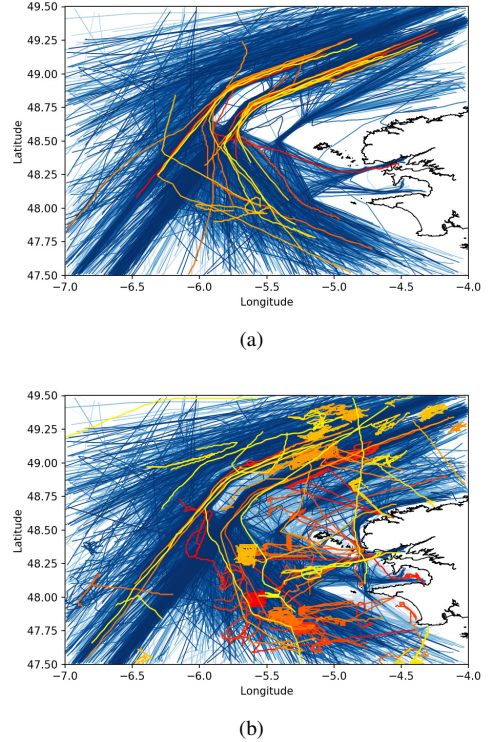
Fig. 11. Anomaly detection examples for a the model trained on the same data as Fig. 10a and tested on data from July 21 to September 30, 2017. (a) When the data comprise only cargo and tanker vessels. (b) When the data comprise all kind of vessels.
