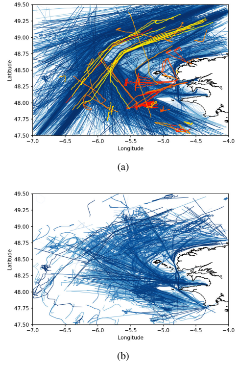
Fig. 10. Anomaly detection examples of KDE GeoTrackNet with AIS data comprising all vessel types from January to March 2017. (a) AIS tracks that are flagged as abnormal by KDE GeoTrackNet . Some tracks are statistically abnormal, however, their behaviors are not suspicious. For examples, the red tracks that steam from land are fishing vessels went fishing; they were detected as abnormal because there were not enough similar AIS tracks in the training set. (b) AIS tracks of fishing vessels in the training set (about 13% of tracks in the training set).
