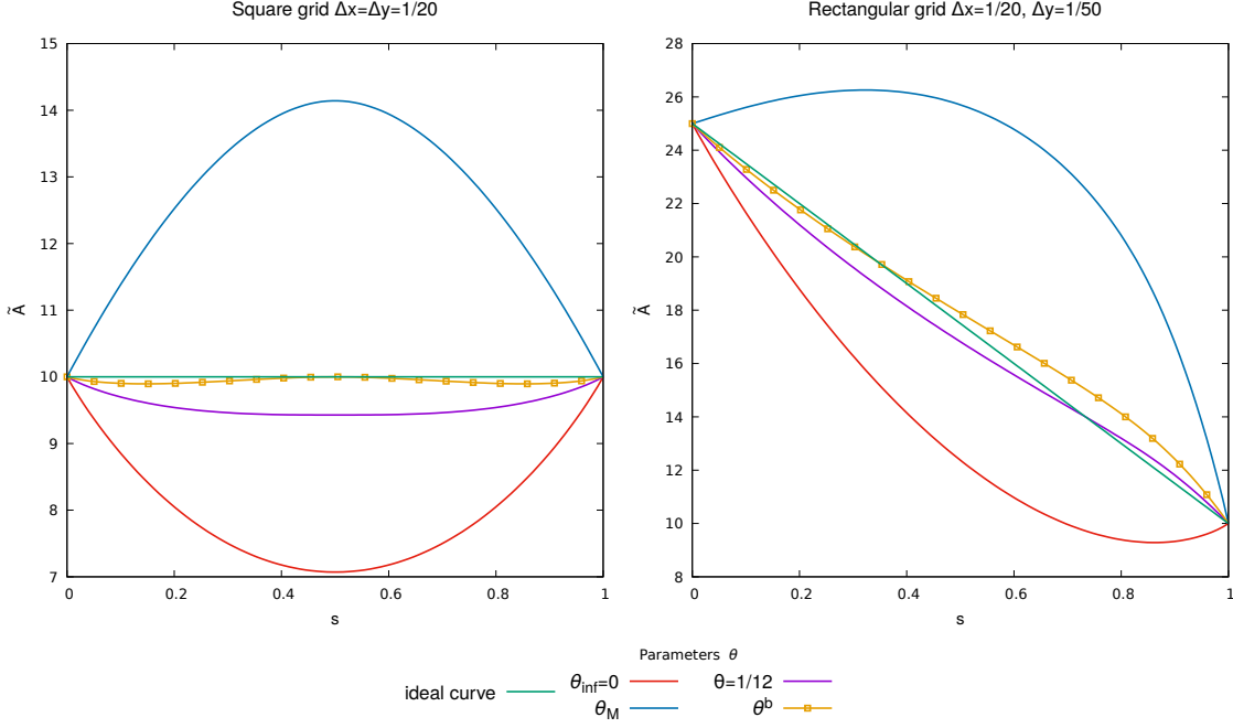
Figure 4: Angular error associated with the 9P1s scheme s \mapsto \tilde{A}_{\Delta x, \Delta y}^\theta for a few values of \theta . Left panel: z = 1 , \theta_M = 0.5, \theta^b = 0.103553 . Right panel: z = 0.4 , \theta_M = 0.137931 , \theta^b = 0.074967 .
