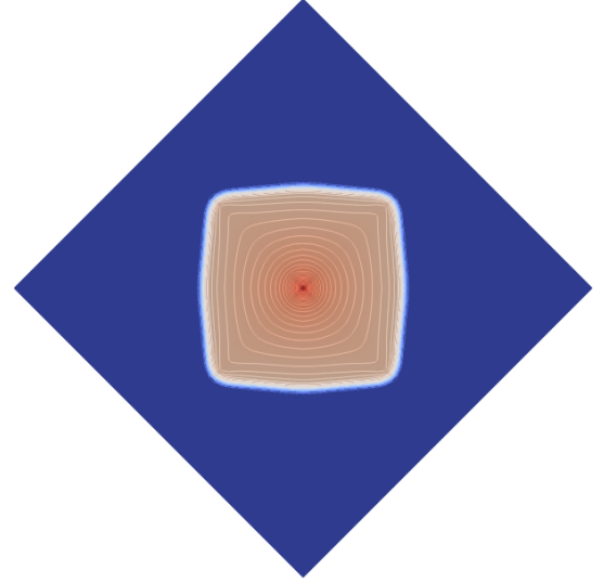
(b) 9P1s scheme with \theta^b and parallel mesh.
