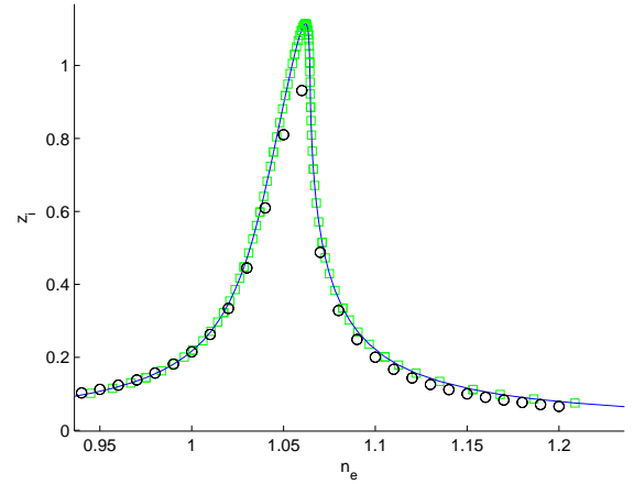
Figure 3. Forced response for \hat{C}_1 = 0.005 computed from Eq. (23), \square : stable, \times : unstable. Comparison with time integration of Eq. (17) and (18) ( \circ )
