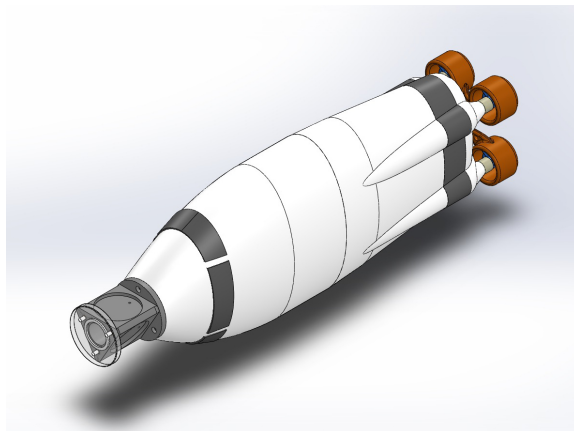
Fig. 4 First design of the aFish (artificial fish).
