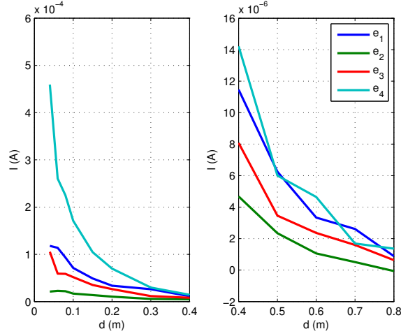
Fig. 10 Raw currents measured on the 4 electrodes of the passive aMussel while increasing the distance between the 2 aMussels.
