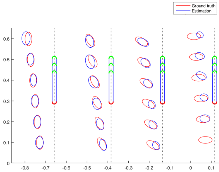
Fig. 14 Localization and estimation of a 33 \times 16 conductive ellipsoid at 5 different distance. Real ellipses (red), estimates (blue).
