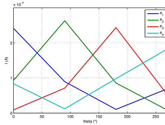
Fig. 9 Raw currents measured on the 4 electrodes of the passive aMussel with 4 different orientations ( 0^\circ, 90^\circ, 180^\circ, 270^\circ ) at the same position.
