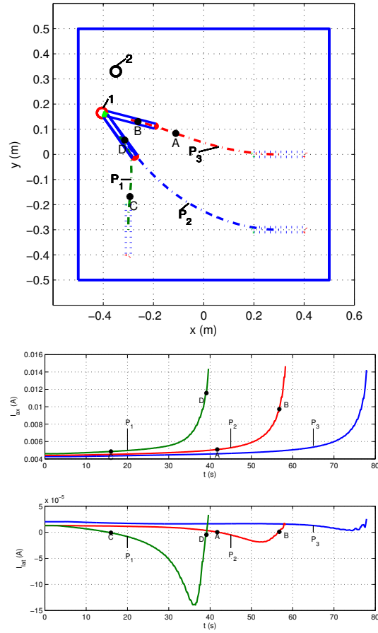
Fig. 12 Starting from 3 different initial poses (dashed lines), the sensor seeks the emitter until it touches it following 3 paths (a) Scene and paths P1, P2 and P3. (b) Axial currents ( I_{ax} ) and (c) lateral currents ( \delta I_{lat} ) for the 3 paths. A, B, C, D indicate poses where the sign of lateral currents change [4].
