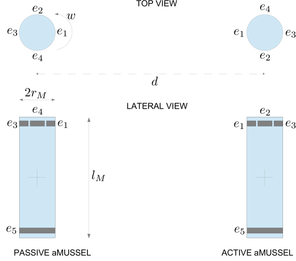
Fig. 8 aMussel experiment set up.
