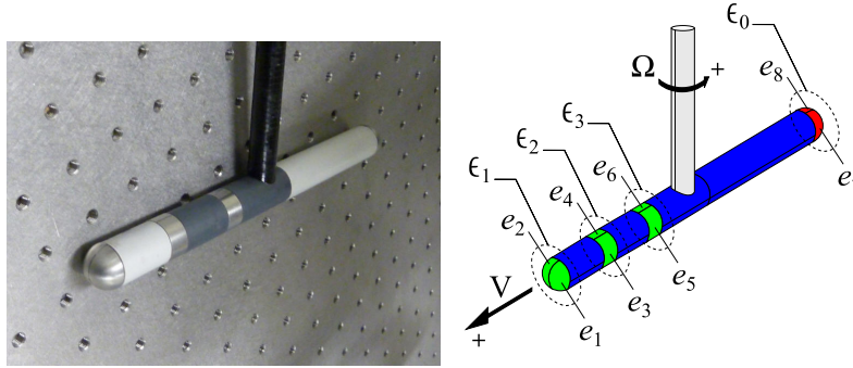
Fig. 7 Left: Artificial electric sensor [17], Right: Design of the sensor with our notations.
