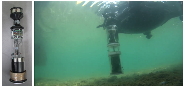
Fig. 3 Left: An aMussel, Right: An aMussel recharging on an aPad.
