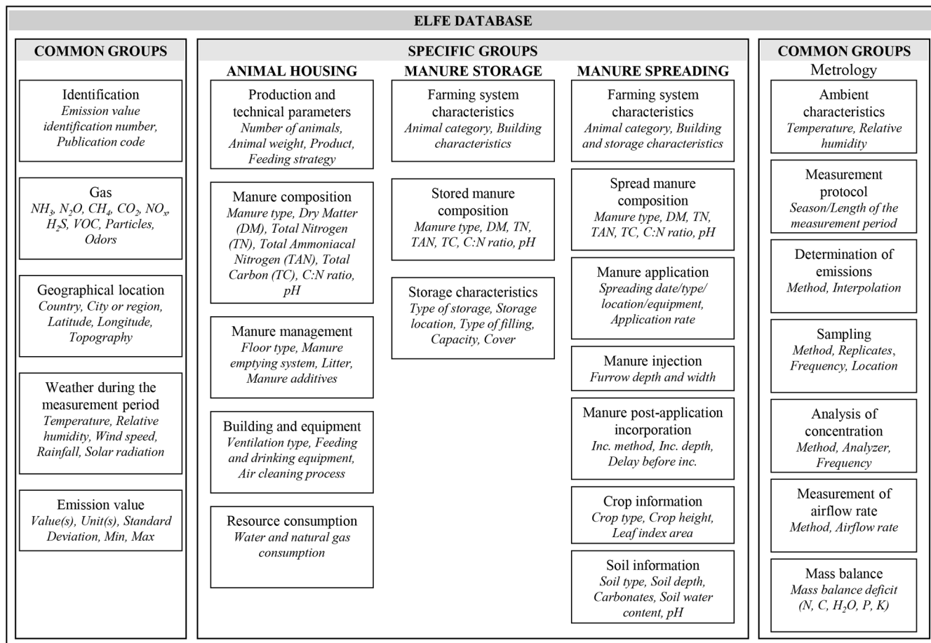
Fig. 1. Organization of thematic groups in the five files of the ELFE (Livestock and Emission Factors) database: Common groups (Files 1–5), Animal housing (Files 1–3), Manure storage (File 4), and Manure spreading (File 5). VOC, volatile organic compound.
