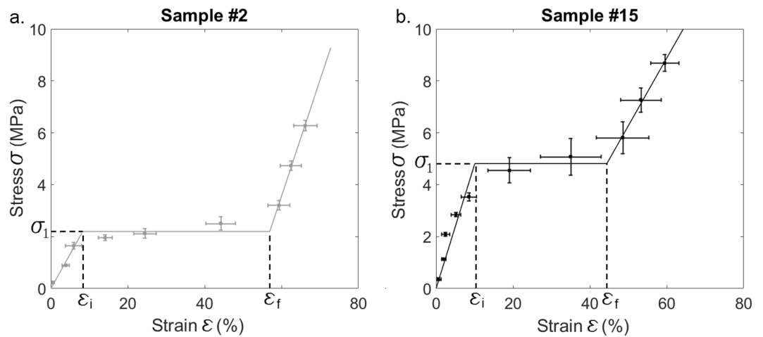
Figure 2. Variation of the stress applied to the bone-implant interface as a function of the strain obtained for bone samples #2 (a) and #15 (b). Parameters \sigma_1 , \epsilon_i and \epsilon_f corresponding to the Neo-Hookean behavior of bone tissue are indicated. The solid lines represent the optimal functions \tilde{\sigma} corresponding to each bone sample.
