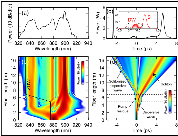
Fig. 1. Numerical simulations showing solitonization of a dispersive wave. (a) Output spectrum and (c) temporal trace after 17 m of propagation. The inset in (c) corresponds to the temporal trace at a fiber length of 7 m, i.e. just after the dispersive wave has crossed the ZDW and has entered the anomalous dispersion region. The dispersive wave (DW) that will be solitonized is surrounded by the dashed black line, and S is the soliton. (b) Spectral and (d) temporal dynamics with fiber length. The black line in (b) is the ZDW. Black dashed lines in (d) depict the start and end of the tapered section.
