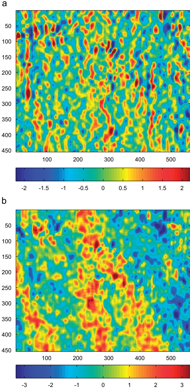
Fig. 17. (u_x - u_{x,average}) maps for two different numerical imposed x displacements (colormap values in percentage of the pitch).
