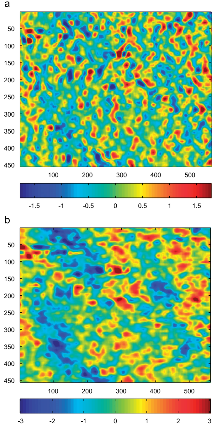
Fig. 18. (u_y - u_{y,average}) maps for two different numerical imposed x displacements (colormap values in percentage of the pitch).
