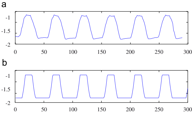
Fig. 6. Profile of the grating for an exposure dose of 1 J/cm 2 . (a) Practical profile; (b) theoretical profile.
