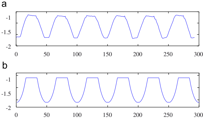
Fig. 5. Profile of the grating for an exposure dose of 500 mJ/cm 2 . (a) Practical profile; (b) theoretical profile.
