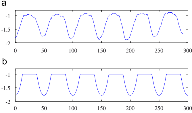
Fig. 4. Profile of the grating for an exposure dose of 300 mJ/cm 2 . (a) Practical profile; (b) theoretical profile.
