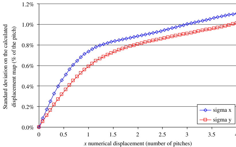
Fig. 16. Standard deviation of the calculated maps of u_x and u_y plotted against the numerical displacement.
