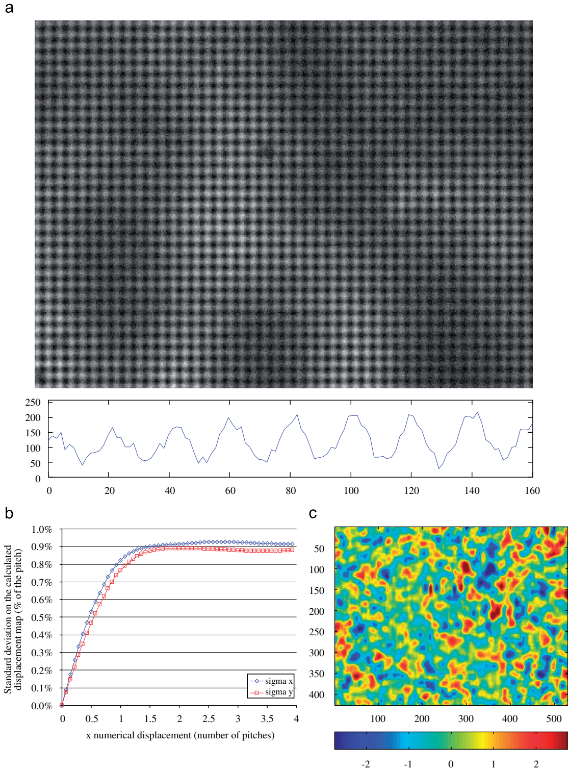
Fig. 19. Results obtained for a simulated grid with variable contrast and white noise: (a) simulated grid; (b) standard deviation plotted against the numerical displacement; (c) (u_x - u_{x,average}) map for an imposed x displacement = 4 \times p (colormap values in percentage of the pitch).
