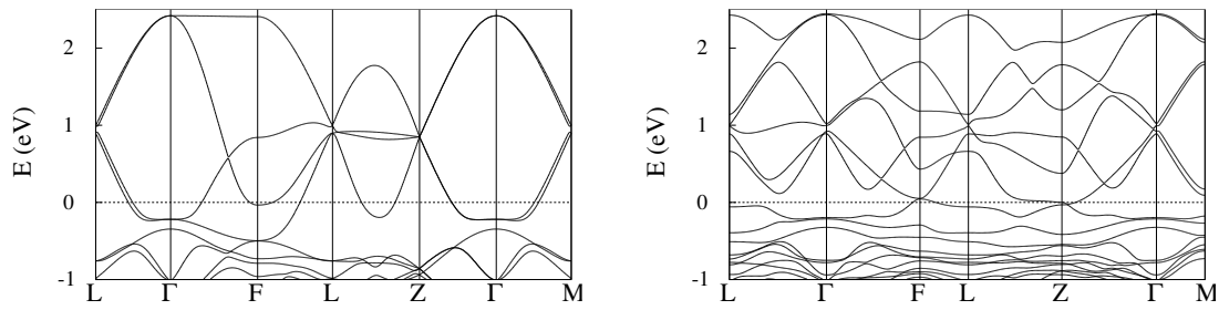
Figure 4: Calculated band structures of the nonmagnetic R\bar{3}c \text{LaNiO}_3 (left) and the disproportionated antiferromagnetic R -type \text{LaNiO}_3 corresponding to the propagation wave vector (0, 0, \frac{1}{2})_r . The band structures are plotted along the path L (\frac{1}{2}, 0, 0)_r \rightarrow \Gamma (0, 0, 0) \rightarrow F (\frac{1}{2}, \frac{1}{2}, 0)_r \rightarrow L (\frac{1}{2}, 0, 0)_r \rightarrow Z (\frac{1}{2}, \frac{1}{2}, \frac{1}{2})_r \rightarrow \Gamma (0, 0, 0) \rightarrow M (0, 0, \frac{1}{2})_r . The coordinates are given in terms of the reciprocal lattice vectors of the primitive cell.
