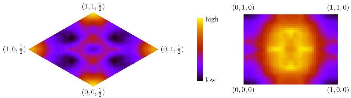
Figure 3: Calculated Lindhard susceptibility of \text{LaNiO}_3 in the R\bar{3}c (left) and Pnma (right) structures.
