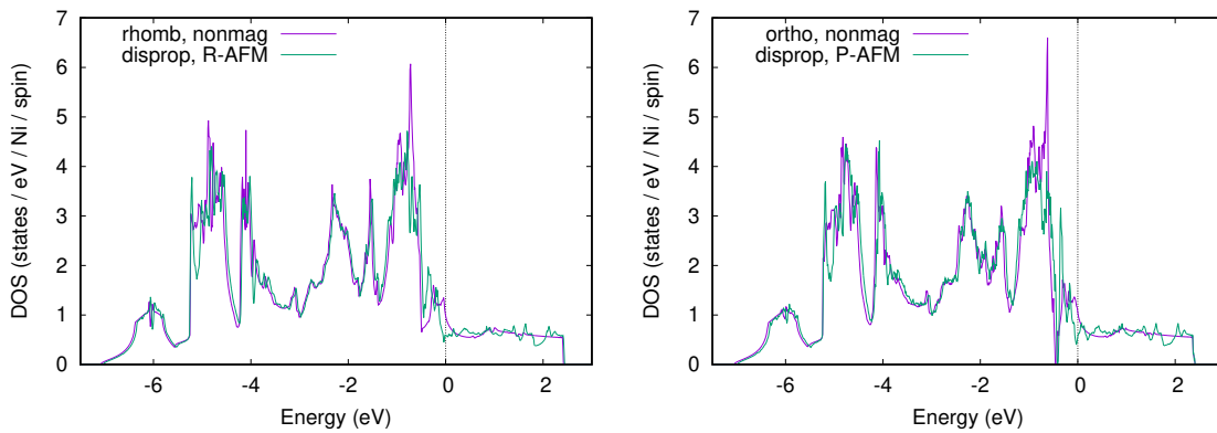
Figure 7: Left: Calculated electronic DOS of LaNiO_3 in the rhombohedral non-magnetic and disproportionated antiferromagnetic R -type structures. Right: DOS of LaNiO_3 in the orthorhombic non-magnetic and disproportionated antiferromagnetic P -type structures.
