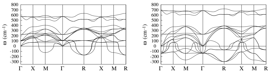
Figure 1: Calculated PBE GGA non-spin-polarized phonon dispersions of cubic \text{LaNiO}_3 (left) and cubic \text{YNiO}_3 (right). The imaginary frequencies are denoted by negative values.
