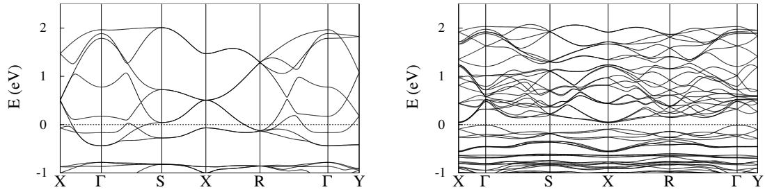
Figure 6: Calculated band structures of the nonmagnetic Pnma YNiO_3 (left) and the disproportionated antiferromagnetic P -type YNiO_3 corresponding to the propagation wave vector (\frac{1}{2}, \frac{1}{2}, 0)_o . The path is as in Fig. 5.
