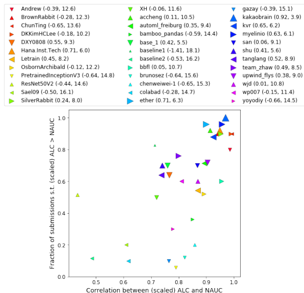
Fig. 6: \%(\text{ALC} > \text{NAUC}) vs \text{correlation}(\text{ALC}, \text{NAUC}) . ALC and NAUC were “scaled” (see text). The numbers in the legend are average scaled ALC and average rank of each participant. The marker size increases monotonically with average scaled ALC.
