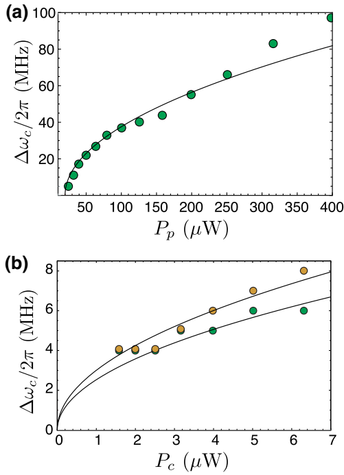
FIG. 3. (a) Parametric locking range \Delta\omega_c measured on resonator a as a function of pump power P_p . The pump frequency \omega_p is set to 2\pi \times 14.95 GHz and the parametric locking tone is injected at \omega_c for a constant power P_c = -20 dBm. The full black line corresponds to \Delta\omega_c \propto \sqrt{P_p} . (b) Parametric locking range measured on the mode a (green dots) and mode b (orange dots) as a function of locking signal power P_c at \omega_c . The pump frequency \omega_p is set to 2\pi \times 14.95 GHz and the pump power P_p is set to -16 dBm. Full black lines correspond to \Delta\omega_c \propto \sqrt{P_c} .
