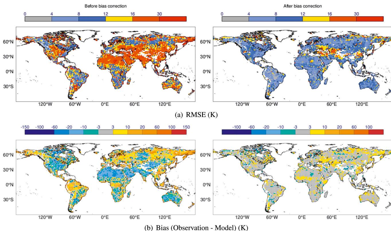
Fig. 9. Comparison between ECMWF CMEM and SMOS TBs before (left) and after (right) bias correction, for 2015, at X pol and 40° incidence angle. Panels a and b show RMSE (K) and bias (K), respectively.
