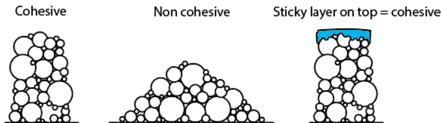
Figure 12. Schematic interpretation of the “sticky layer” effect due to the presence of poorly fractured, consolidated sediments on the top of Variscan basement rocks in the PB.
