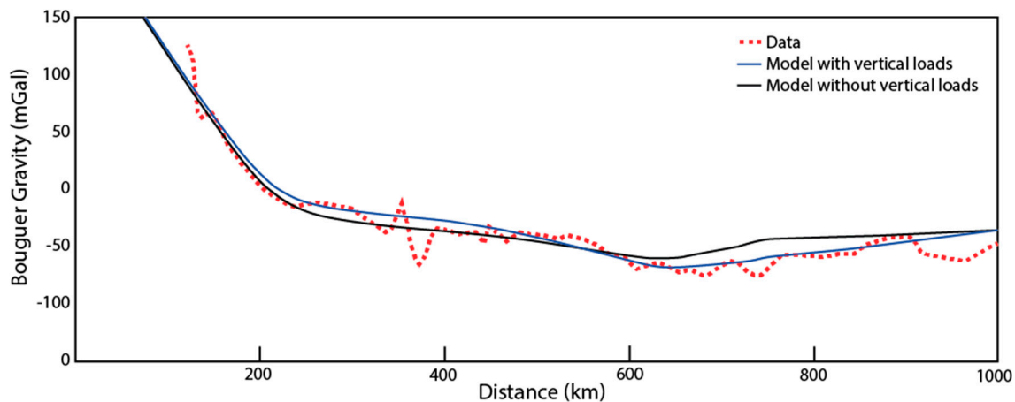
Figure 5. Observed (open red dots) and modelled (solid lines) Bouguer gravity along the profile for a model without additional line loads (i.e., with only elastic compensation of the topographic load, in black) and with line loads applied at km 400 and 750 (in blue).
