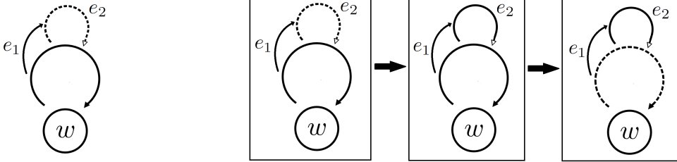
Figure 1: Example and evolution of a switch graph.
