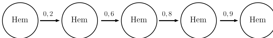
Figure 6: Non-reactive weighted model for hemoglobin protein.
