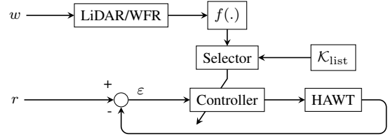
Fig. 1: On-line implementation of the controller selection framework. r refers to the set point, \varepsilon to the regulation error and w is the wind.
