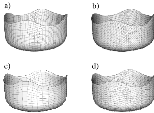
Fig. 15. Final deformed shape for a completely drawn cylindrical cup using a) the SHB8PS elements; b) the SHB6 elements; c) the SHB20 elements; and d) the SHB15 elements
