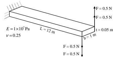
Fig. 3. Elastic cantilever beam subjected to torsion-type loading
