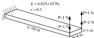
Fig. 2. Elastic cantilever beam subjected to bending forces
