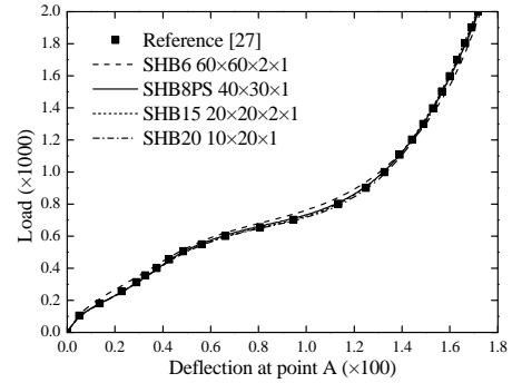
Fig. 9. Load–deflection curves for the pinched semi-cylindrical shell
