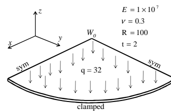
Fig. 6. Clamped circular plate
