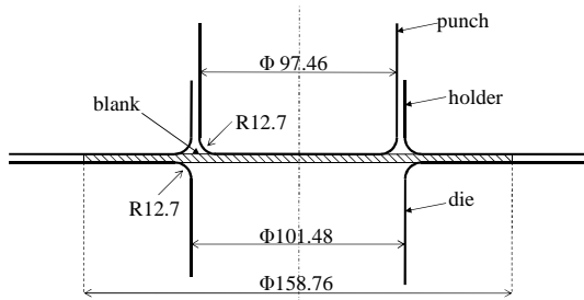
Fig. 14. Schematic view of the drawing setup [29]
