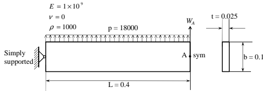
Fig. 12. Simply supported elastic beam
