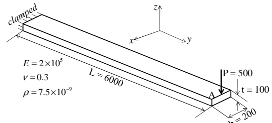
Fig. 10. Elastic cantilever beam under impulsively-applied loading
