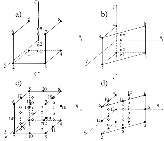
Fig. 1. Reference geometry of the SHB elements and location of their integration points: a) linear hexahedral SHB8PS element; b) linear prismatic SHB6 element; c) quadratic hexahedral SHB20 element, and d) quadratic prismatic SHB15 element
