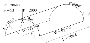
Fig. 8. Pinched semi-cylindrical shell
