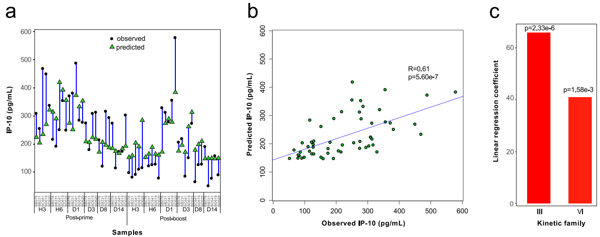
Figure 6. Association of kinetic families with a direct biological measurement. (a) The relationship between kinetic family abundances and IP-10 plasma concentration was analyzed using linear regression. Iterative linear regressions were generated until all coefficients had a p-value \leq 0.05 . At each iteration, the coefficient having the highest p-value higher than 0.05 was removed. The differences between predicted vs. observed concentrations of IP-10 are shown. (b) The ELISA measured and linear regression predicted IP-10 concentrations are shown in a bi-plot representation. The Pearson correlation coefficient and p-value are indicated. (c) The linear regression coefficients of kinetic families III and VI, which are necessary and sufficient to predict IP-10 concentrations, are displayed along with their p-values.
