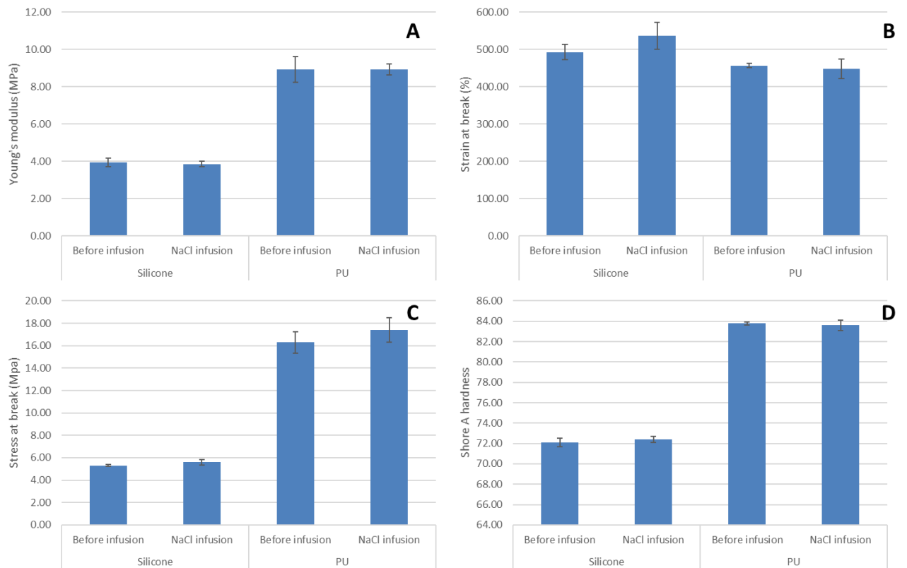
Figure A : Mechanical properties (A = Young's modulus; B = strain at break; C = stress at break; D = Shore A hardness) of polyurethane (PU) and silicone catheters before and after infusion of a 0.9% NaCl solution (Mean \pm 95% confidence interval, n = 3).
