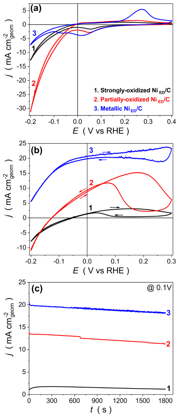
Figure 2. (a, b) CV and (c) chronoamperometry curves obtained for various \text{Ni}_{\text{ED}}/\text{C} rotating disc electrodes (RDE) under \text{N}_2 atmosphere at the following conditions: (a) 1.0 M NaOH, v = 20 mV
