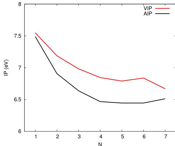
Figure 6: Vertical and adiabatic ionization potential of pyrene clusters
