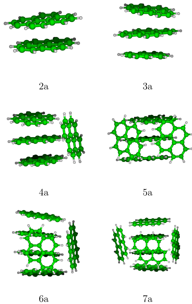
Figure 5: Most stable structures of cationic pyrene clusters.
