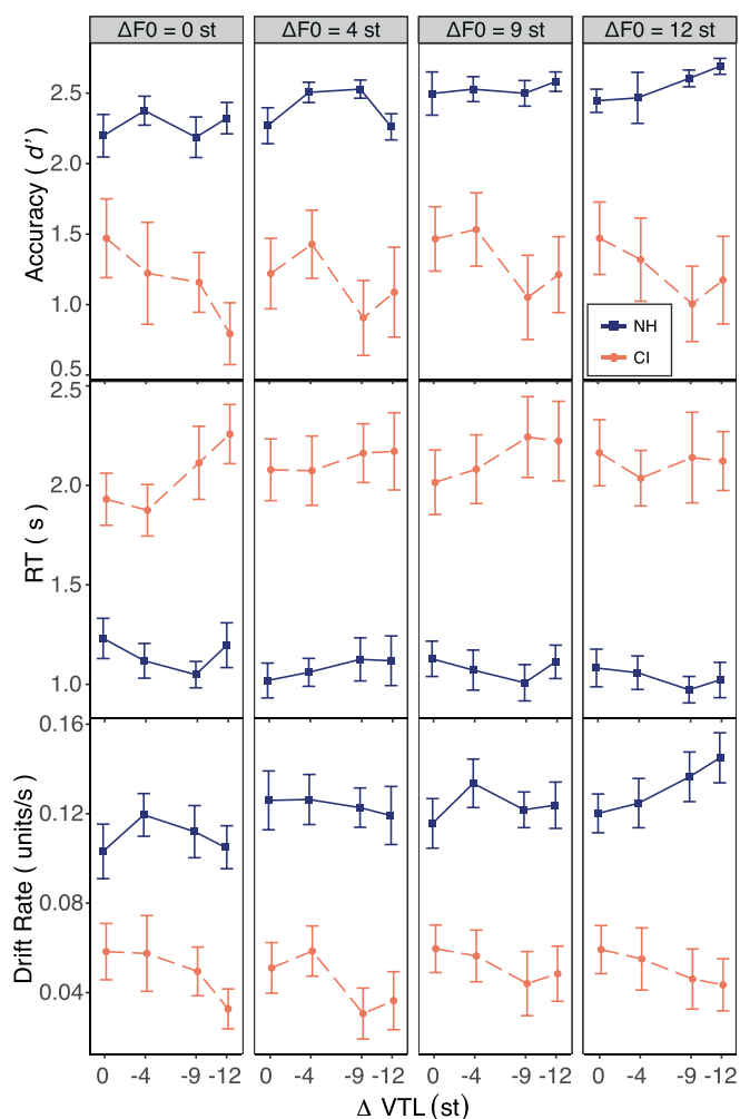
FIG. 4. (Color online) SoS comprehension performance, measured using SVT, averaged per group for each condition of \Delta F0 (different panels) and \Delta VTL ( x axis). Dark squares with solid lines represent the NH data, while light circles with dashed lines represent the CI data. Error bars represent one standard error from the mean. (Top row) SoS comprehension accuracy measured in d' . (Middle row) SoS comprehension RTs measured in seconds. (Bottom row) SoS comprehension drift rate measured in arbitrary units per second.
