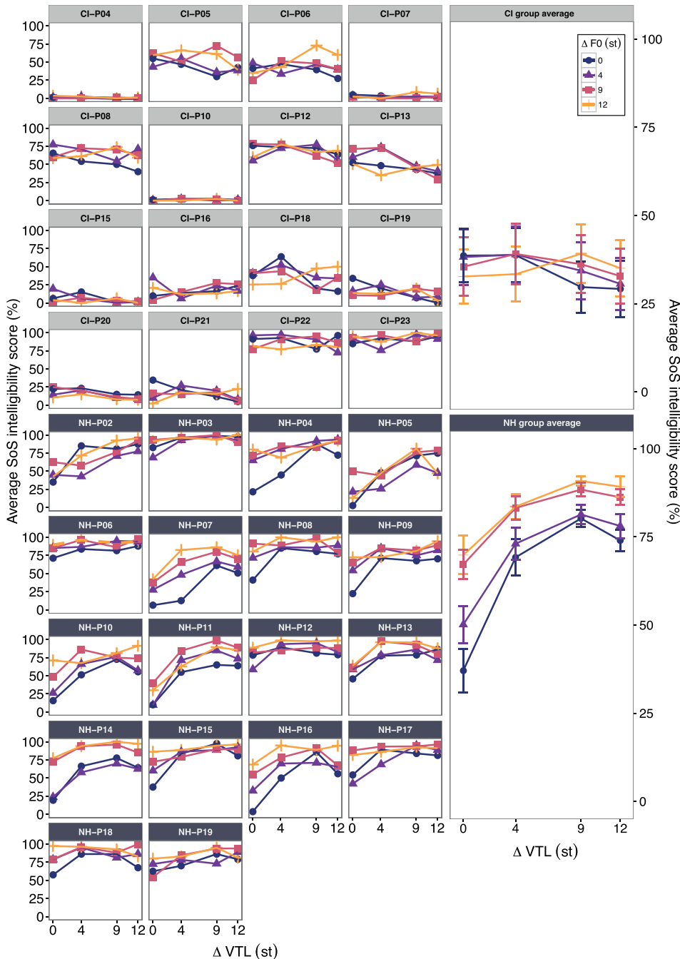
FIG. 8. (Color online) Individual (small panels) and group (large panels) SoS intelligibility scores (experiment 1) plotted against \Delta VTL for each value of \Delta F0 . (Top) (light labels) CI data. (Bottom) (dark labels) NH data.
