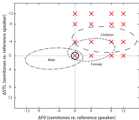
FIG. 1. (Color online) [\Delta F_0, \Delta VTL] plane. The reference female speaker is at the origin of the plane, as indicated by the solid circle. Decreasing F_0 and elongating VTL yields deeper-sounding male-like voices, while increasing F_0 and shortening VTL yields child-like voices. Dashed ellipses, derived from the data of Peterson and Barney (1952), indicate the ranges of typical F_0 and VTL differences between the reference female speaker from experiment 1 and 99% of the population. The data of Peterson and Barney were normalized to the reference female speaker in experiment 1. The red crosses indicate the 16 different combinations (experimental conditions) of \Delta F_0 and \Delta VTL used in both experiments 1 and 2.
