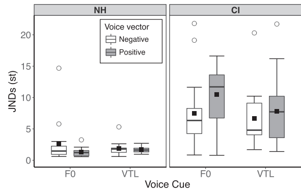
FIG. 5. F_0 and VTL JNDs for NH (left) and CI (right) listeners. Positive (shaded bars) and negative (empty bars) voice vectors denote the principal axes of the [\Delta F_0, \Delta VTL] plane in Fig. 1, which refer to vectors from the origin along positive and negative values, respectively, of F_0 and VTL. The boxes extend from the lower to the upper quartile, and the middle line shows the median. The whiskers show the range of the data within 1.5 times the interquartile range (IQR). The filled squares show the means, while the empty circles show the individual data outside of 1.5 times IQR.
